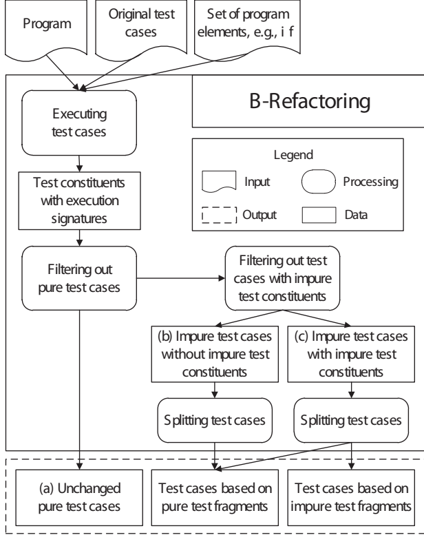
Fig. 2. Conceptual framework of B-Refactoring. This framework takes a program with test cases and a specific set of program elements (e.g., if elements) as input; the output is new test cases based on test fragments. The sum of test cases in (a), (b), and (c) equals to the number of original test cases.
